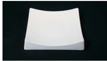
35 225 61 NEU / NEW Fusingform Teller eckig Ad:15 / Id:15 / H: 2.5 cm Fusing mold square plate Od:15 / Id:15 / H: 2.5 cm
